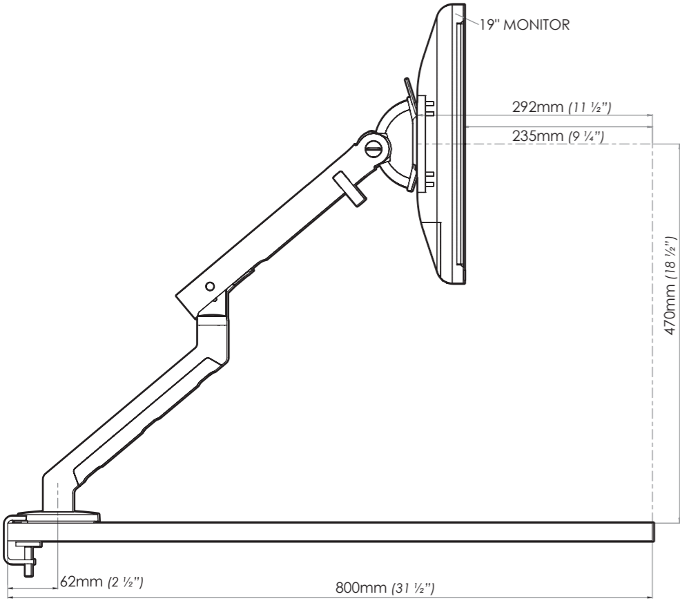
UPPER POSITION
