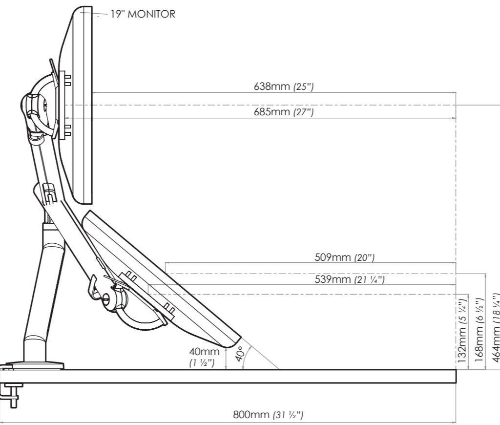
FORWARD POSITION
