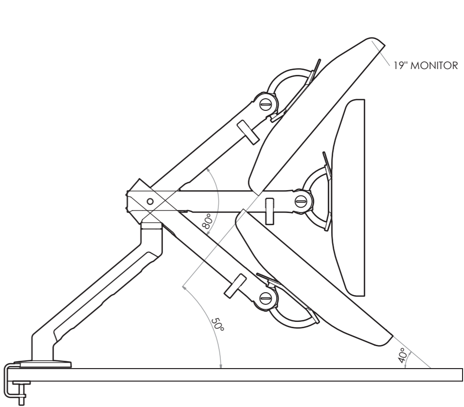
REAR POSITION
